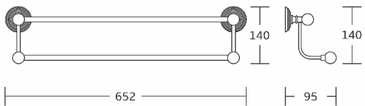
15125 Double towel bar Material:Stainless steel 304 Size:652x140x95mm
