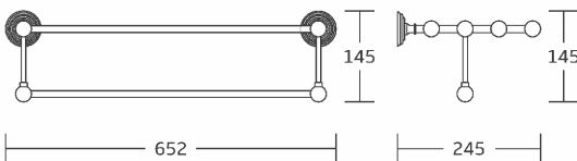
15120 Towel shelf Material:Stainless steel 304 Size:652x145x245mm
